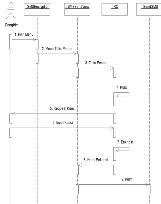
Gambar 3.6 Sequence Diagram Pengirim Pesan
