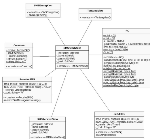
Gambar 3.5 Class Diagram RC6
