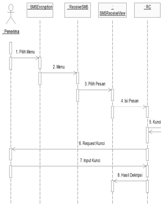
Gambar 3.7 Sequence Diagram Penerima Pesan
