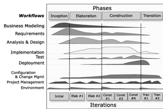
Gambar 2.4 Arsitektur Rational Unified Process (RUP) (10)
